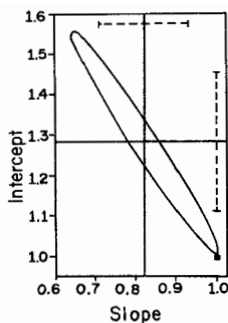
FIGURE 1 Confidence-interval ellipse for a linear least-squares analysis of simulated data.
