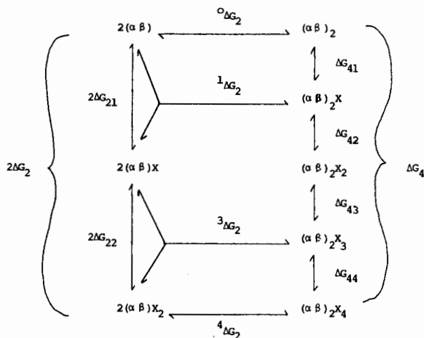
Figure 1.: Linkage diagram for subunit dissociation and oxygenation of human hemoglobin. The energetic quantities represented have been defined previously (7). {}^0\Delta G_2 and {}^4\Delta G_2 are free energies for tetramer formation (from dimers) in the unliganded and fully liganded states, respectively. {}^1\Delta G_2 and {}^3\Delta G_2 are respective association energies for formation of singly liganded tetramer (from combination of singly-liganded and unliganded dimers) and triply-liganded tetramer (from combination of singly and doubly-liganded dimers). Energies for the successive binding steps to tetramer are \Delta G_{41} , \Delta G_{42} , \Delta G_{43} , \Delta G_{44} . For dimer, the successive free energies of oxygenation are \Delta G_{21} and \Delta G_{22} . The free energies for saturation of tetramer and dimer, respectively, are \Delta G_4 and \Delta G_2 . The successive differences ( {}^1\Delta G_2 - {}^0\Delta G_2 ), ( {}^3\Delta G_2 - {}^1\Delta G_2 ), ( {}^4\Delta G_2 - {}^3\Delta G_2 ) are measures of the intersubunit contact energy changes accompanying the first, middle two, and last binding steps, respectively.
